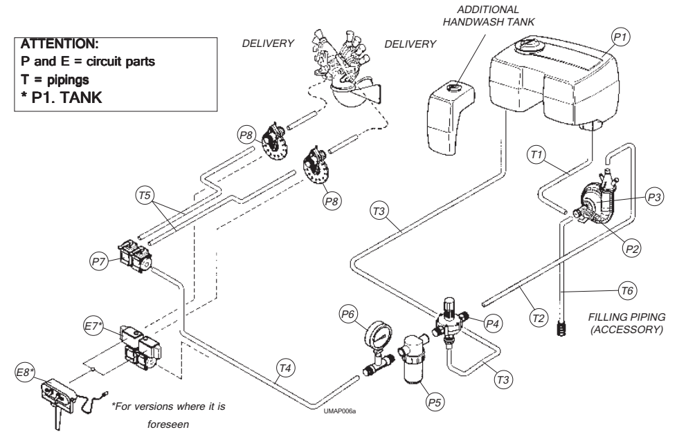
Hydraulic connection diagram
