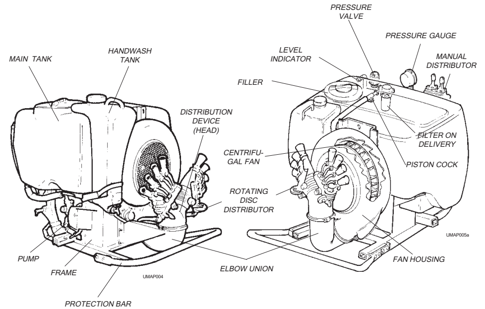
The pictures show the position of the main components of the atomizer.
