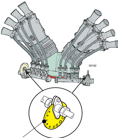
CALIBRATION DISC
